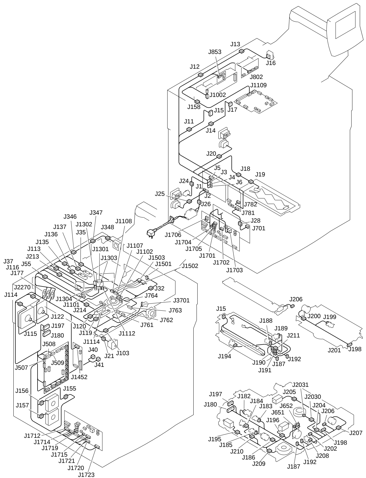
FIGURE B LIST OF CONNECTORS(2/4)
